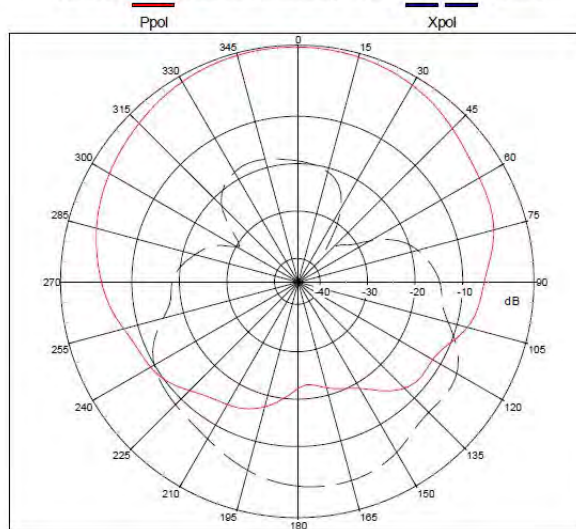
Far-field Pattern @ Phi=90 deg(E-Theta Plane-Cut) Plot Peak Gain= 4.65 dBi; Co-Pol Efficiency: 73.69% @ Freq: 0.86700 GHz
