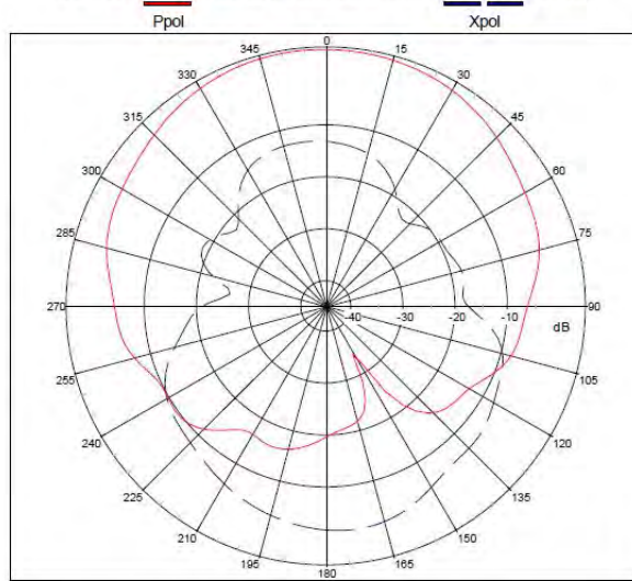
Far-field Pattern @ Phi=0 deg(E-Theta Plane-Cut) Plot Peak Gain= 4.55 dBi; Co-Pol Efficiency: 73.69% @ Freq: 0.86700 GHz
